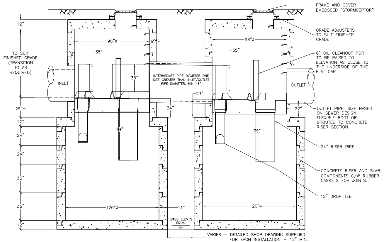
SECTION VIEW
