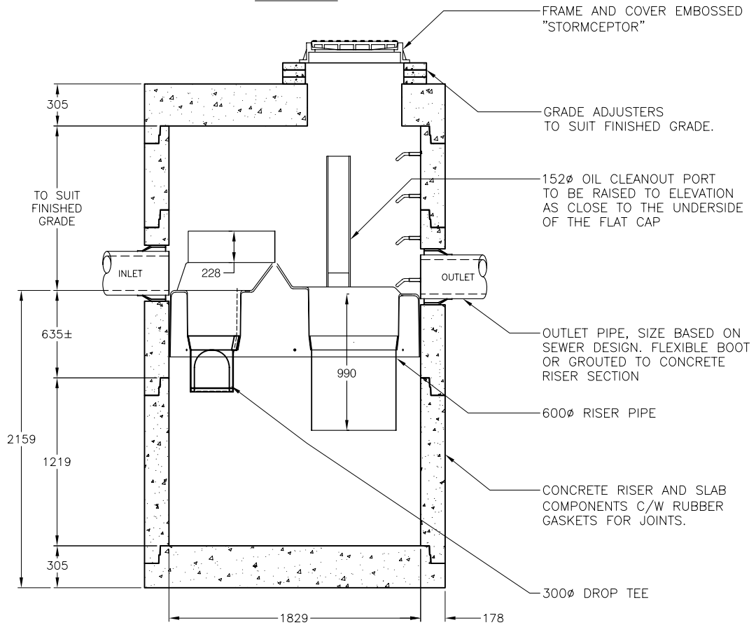
SECTION VIEW
