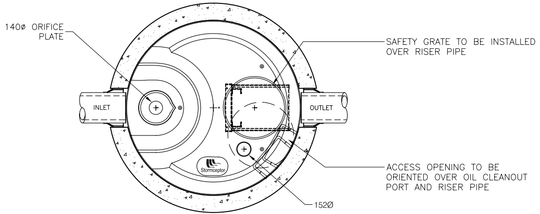
PLAN VIEW
