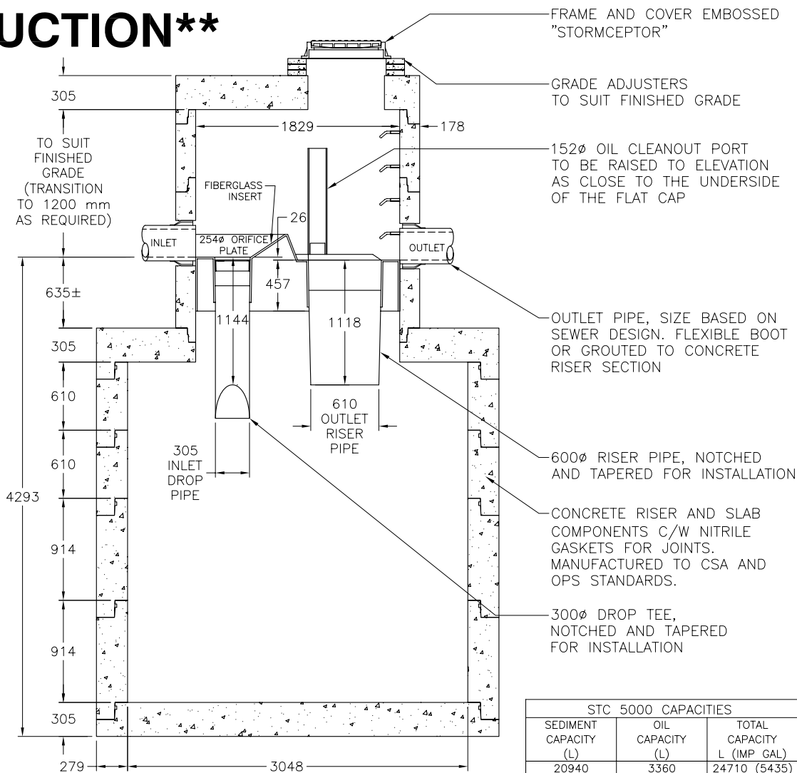
SECTION VIEW
